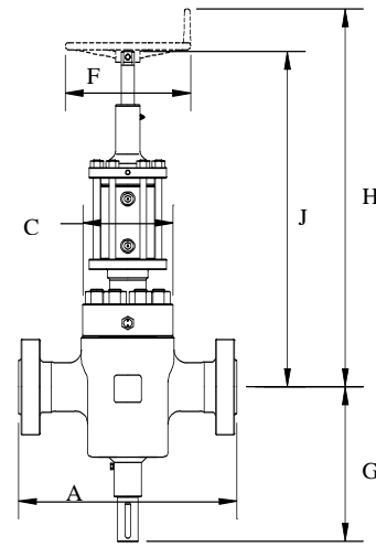
HYDRAULIC GATE VALVE
